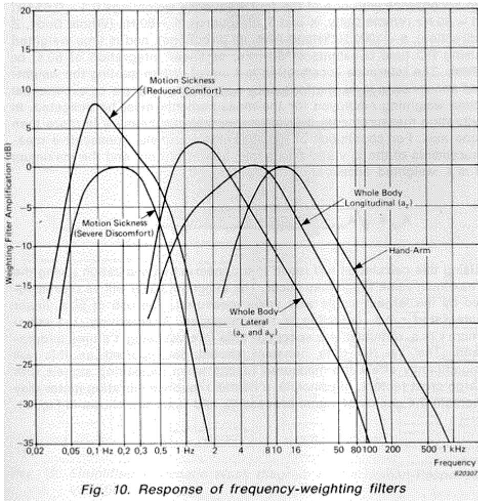
Fig. 10. Response of frequency-weighting filters
