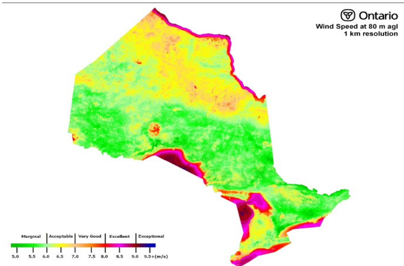
Map 1: Ontario Mesoscale Wind Speed Map
